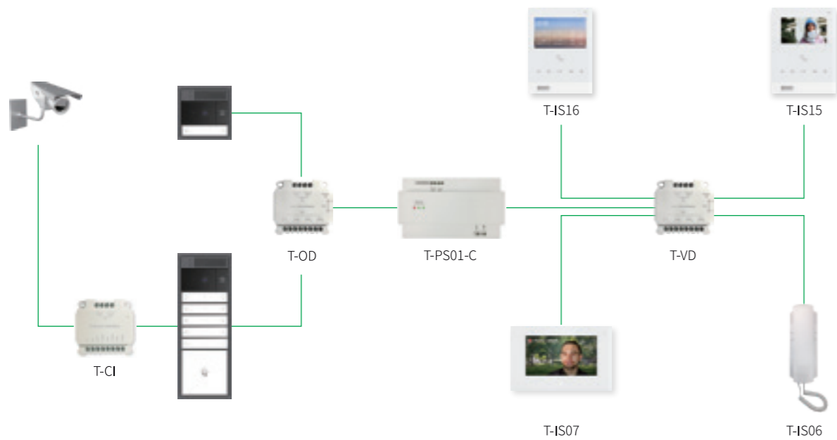
Star Connection:
