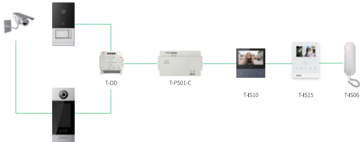
Daisy-chain Connection:
